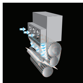
AIR BLOW PAPER SEPARATOR: delivering air prevents the paper from wrapping around the upper fusing belt, thereby improving the reliability of the fusing unit's paper feeding.
